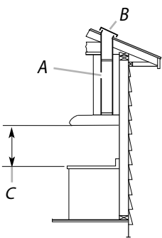
Roof venting
