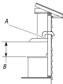
Wall venting
