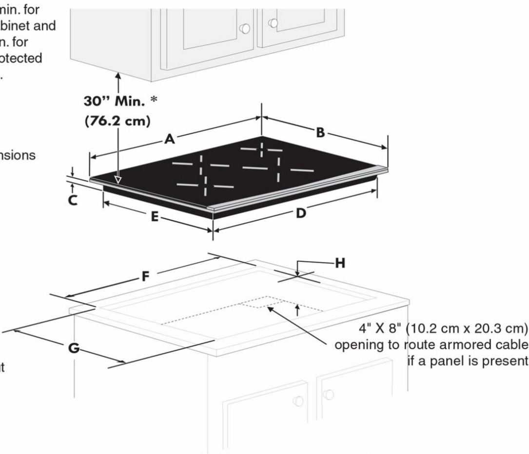
Cooktop Cutout Dimensions
