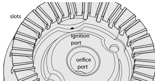
Figure 25: Gas burner head parts
