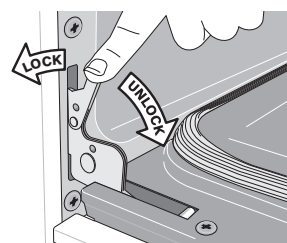
Figure 22: Door hinge locks
