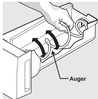
Adjusting Ice Bin Auger
